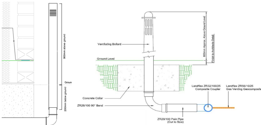
Indicative Gas Venting Bollard Layout Diagrams
